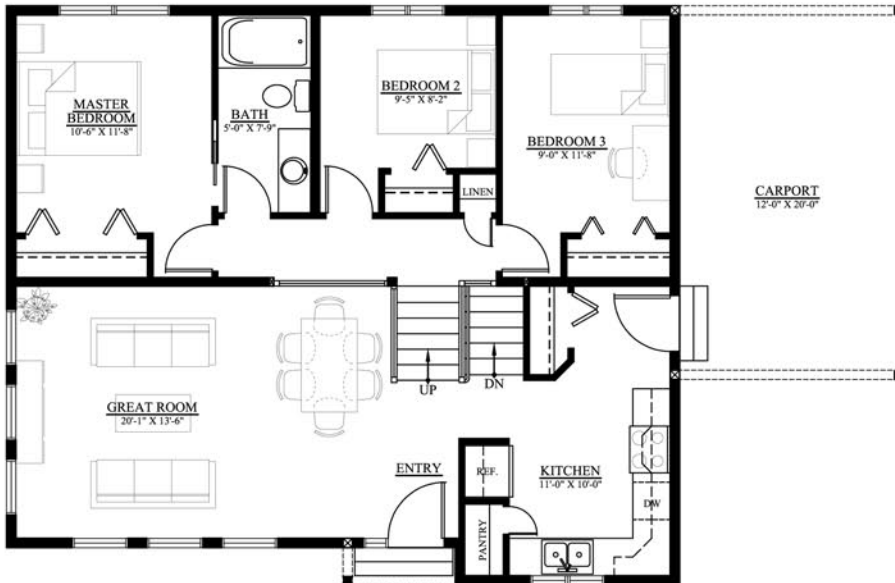
MAIN FLOOR PLAN 1068 SQ. FT
